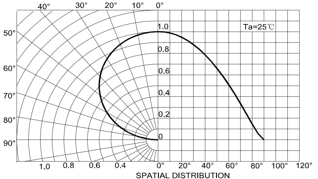
Radiation diagram
